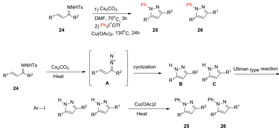
Scheme 6: Synthesis of pyrazoles with copper acetate
