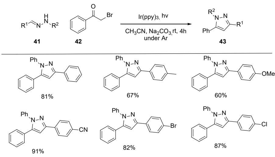
Scheme 13: Synthesis of substituted pyrazoles with \text{Ir(ppy)}_3 catalyst
