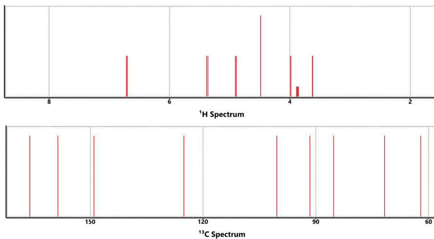
Figure 6. Calculated ^{13}\text{C} and ^1\text{H} NMR spectra for Gemcitabine
