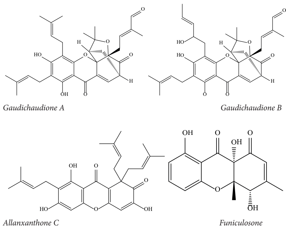
Figure 3. Chemical structures of some bioactive compounds, including the xanthene skeleton.
