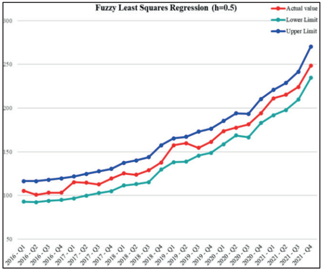
Figure 16. Graphical representation for the fuzzy LSR model for h=0.5
