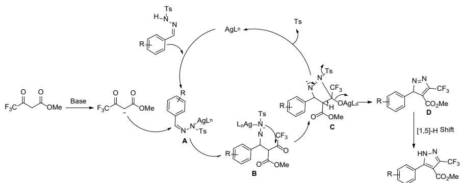
Scheme 10: Synthesis of pyrazole with silver salt
