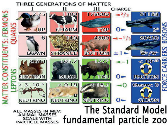
Figure 1. Particle Zoo (Arnaud,2015).
