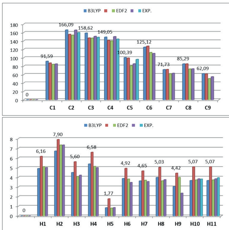
Figure 5. ^{13}\text{C} and ^1\text{H} NMR values for Gemcitabine
