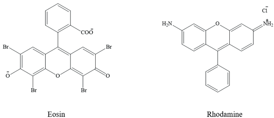
Figure 2. Eosin ve Rhodamine Structures.
