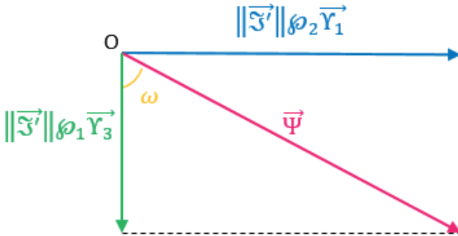
Figure 1. The Darboux vector of (\vec{\mathfrak{S}})
