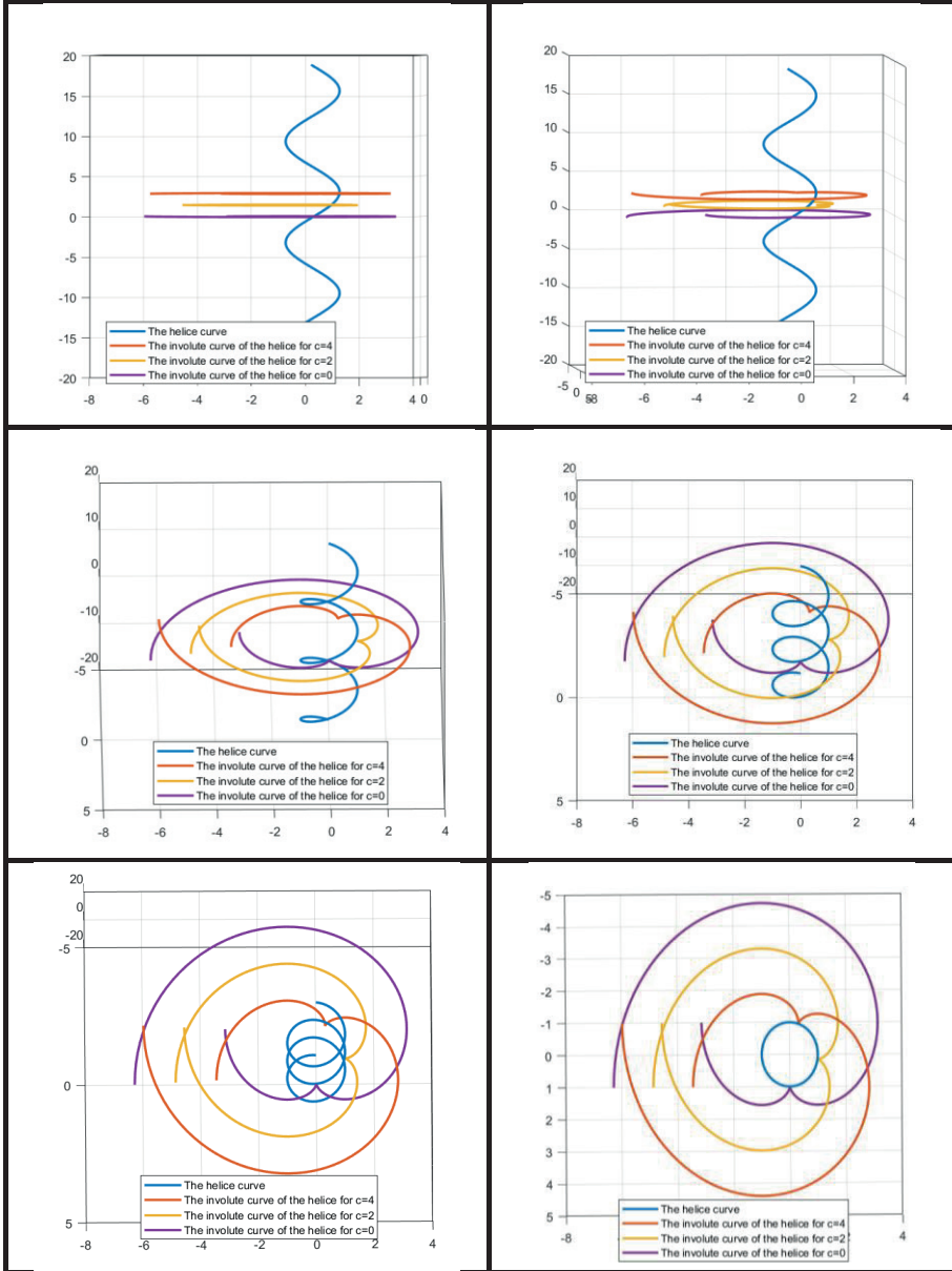
Figure 3. The helix curve (\vec{\mathfrak{S}}) and its three involute curves for c = 0, 2, 4
