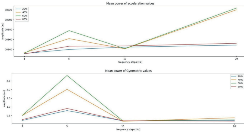
Figure 11. Average power values of vibrations.
