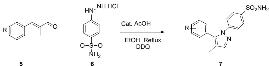
Scheme 2: Synthesis of celecoxib derivatives pyrazoles acid-promoted
