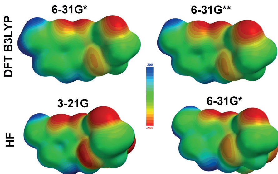
Figure 4. Electrostatic Potential Map (ESPMap) of Gemcitabine
