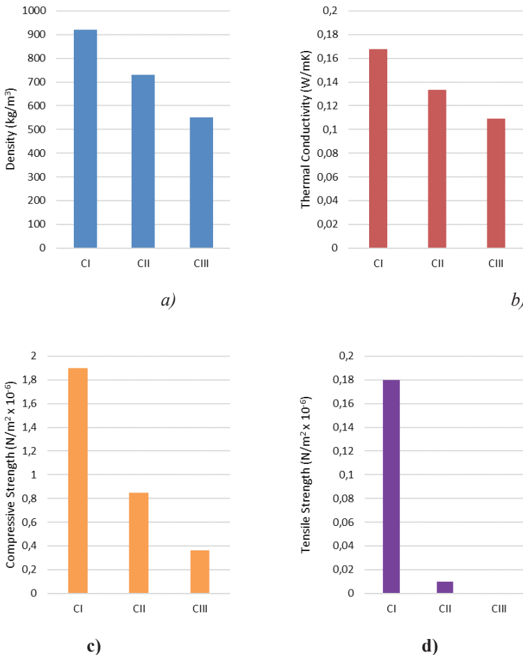
Fig. 2 Physical properties of the concretes with RH aggregate a) Density, b) Thermal conductivity, c) Compressive strength, d) Tensile strength
