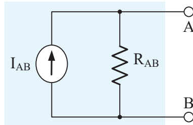
Figure-31. Norton Equivalent Circuit General Notation
