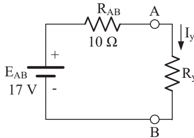
Figure-48 R_3 Connected Thevenin Equivalent Circuit
