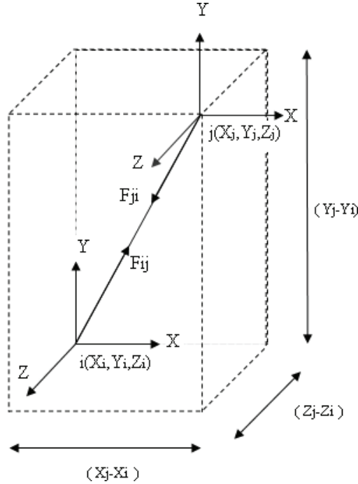
Figure 2. Member i-j of Truss
