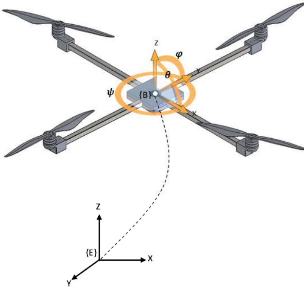
Figure 1. A quadrotor UAV structure
