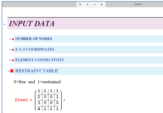
Figure 9. Freedom or restraint conditions of nodes
