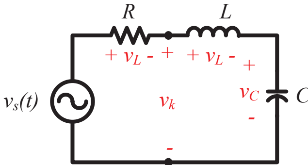
Figure 5. Time domain representation of a lossy circuit
