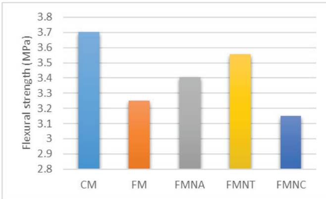
Figure 8. Flexural strength of prisms mortars at 28 days.
