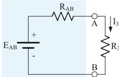
Figure-22 R_3 Connected Thevenin Equivalent Circuit
