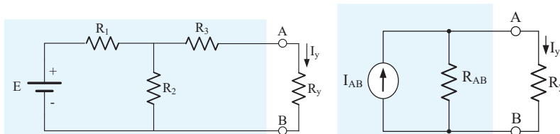
Figure-32. a) Original Circuit b) Norton Equivalent Circuit
