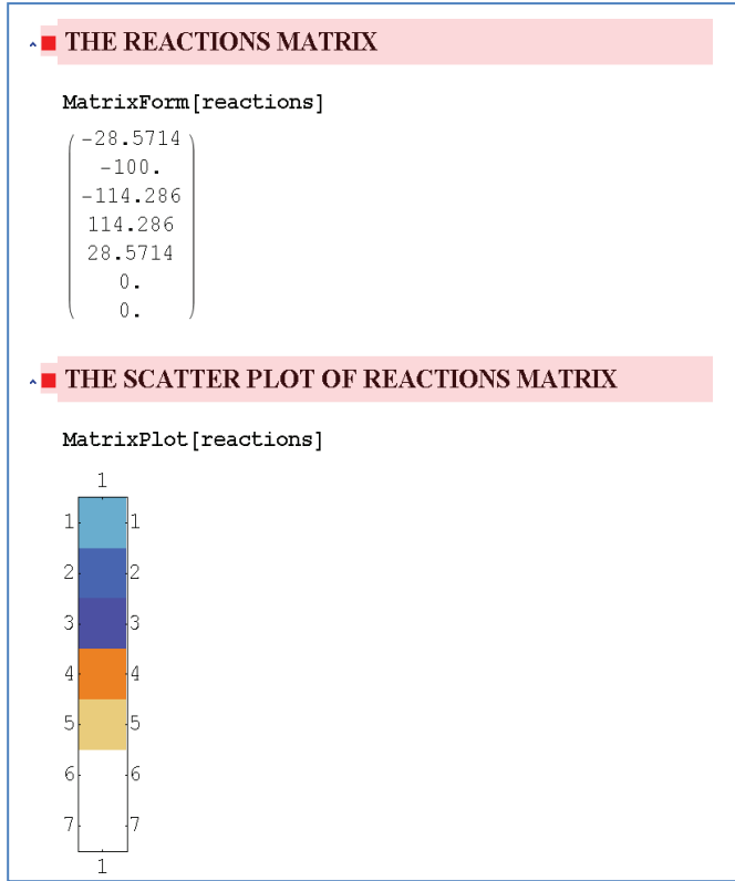
Figure 15. Supports reactions (KN)
