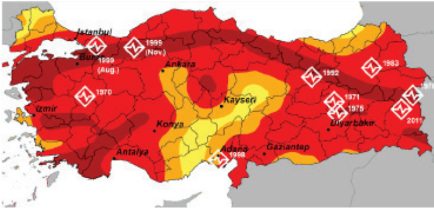
Map 1. Earthquake zones map in Turkey (AFAD, 2011).
