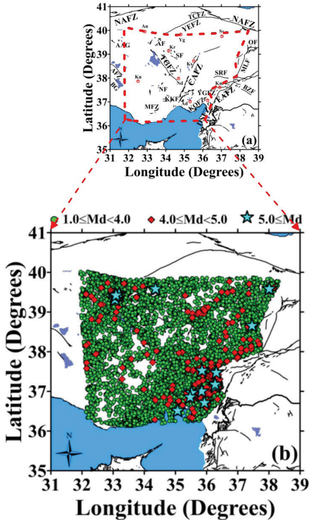
Figure 1. (a) From Arolu et al. (1992), Bozkurt (2001), and Ulusay et al., (2004) simplified tectonic settings. The text included the names of the faults, and the picture included some of the provinces in and around the research region. A: Ankara Yozgat, Sivas, and Kn: Konya, Ks: Kayseri, Kr: Krşehir Nd: Negate, Km: Karamamaraş, Os: Osmaniye, and Ad: Adana. (b) Epicenter distributions for the (Central Anatolia Region) CAR and its surroundings from the original dataset, which included 16,702 shallow earthquakes with M_d \geq 1.0 from 1974 to 2019. The magnitude values of the occurrences were represented by several indicators (Öztürk, 2020).
