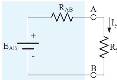
Figure-17 Load Connected Thevenin Equivalent Circuit The current through resistor R_y here is,
