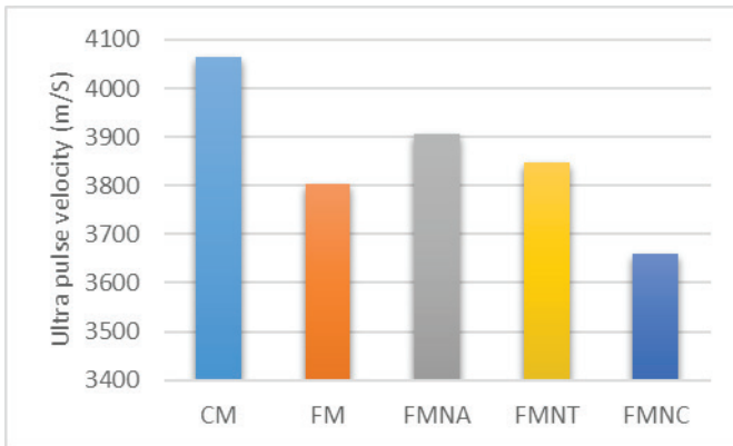
Figure 1. UPV transmission speed of samples at 28 days.
