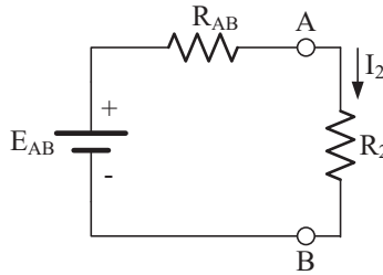
Figure-30 Thevenin Equivalent Circuit Connected to R_2
