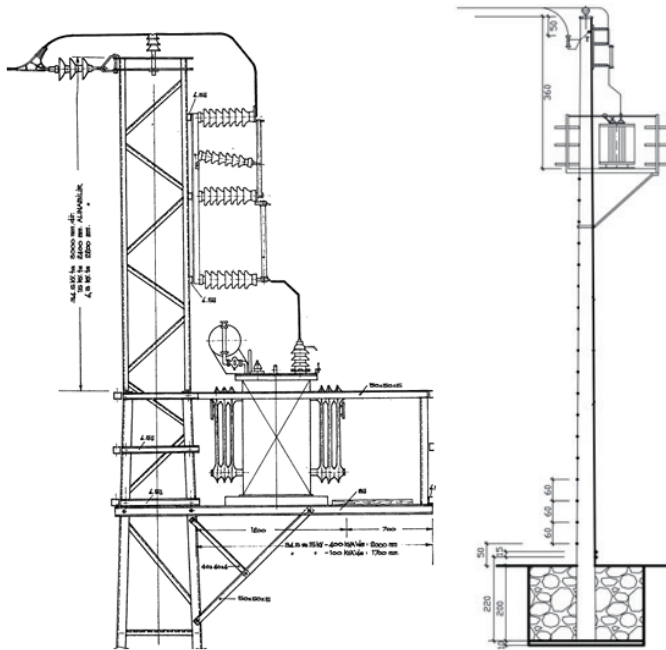
Figure 12. Technical drawing of MV concrete and iron transformer pole [6]
