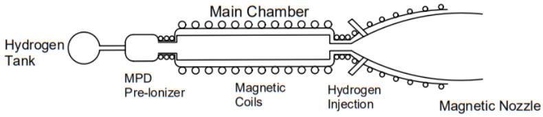
Figure 10. Variable specific-impulse plasma
