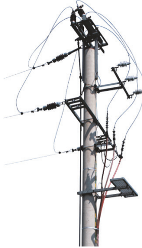
Figure 18. Centrifugal type round (SBA) concrete poles [12]
