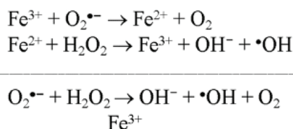
Figure 3. Fenton reactions (Rammouz et al., 2011).
